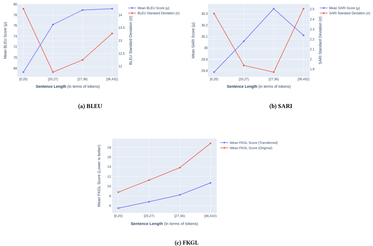
Figure 2: Plots illustrating sentence-length based transfer analysis
