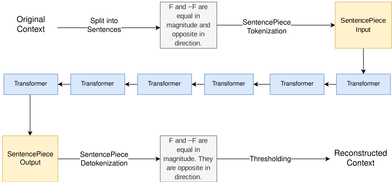
Figure 1: Style Transfer Architecture
